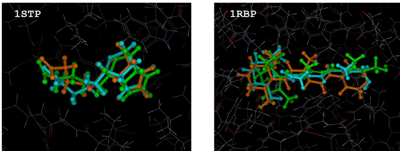
Figure 2 Superimpositions of the X-ray ligand and docked ligand poses to the 1STP and 1RBP complexes. The X-ray ligand is shown in green; the docked ligand using the all-atom model is shown in orange; and the docked ligand position derived from the polar-hydrogen model is shown in cyan, where the non-polar hydrogens were artificially added in the representation.
